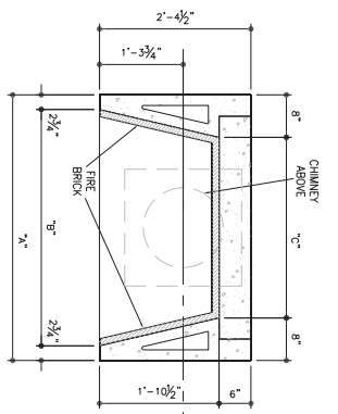
FIREBOX PLAN SCALE: 1" = 1'-0"
