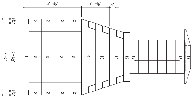
FRONT ELEVATION 42" SYSTEM SCALE: 1" = 1'-0"
